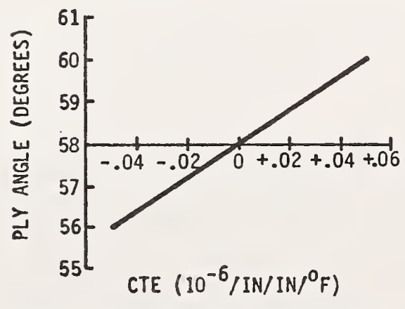
FIGURE 5 : T50(PAN)/T300 ORTHOTROPIC LAMINATE CTE SENSITIVITY
